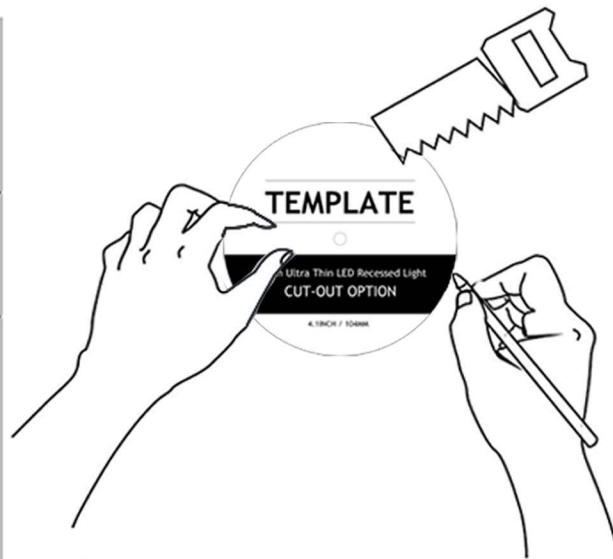
2. Draw the size of panel lamp with 1:1 paperboard and cut out the shape according to the track
